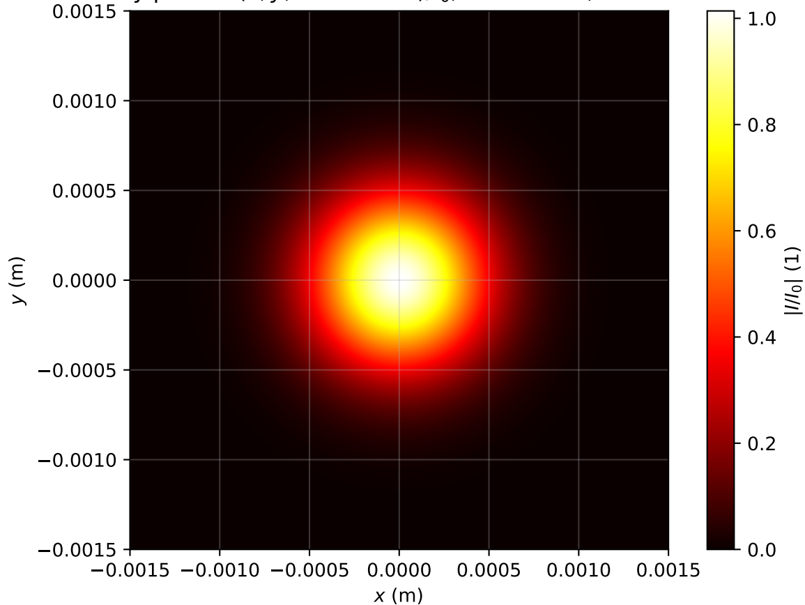
Intensity profile I(x, y, z = 0.159m)/I_0 , Pin=0.8Pcr, artificial time
